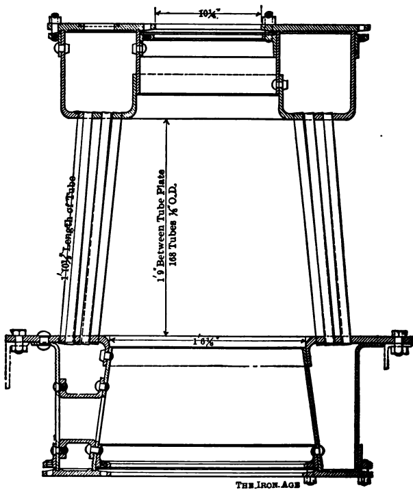
FIG. 342.—The Thornycroft Steam Wagon Boiler.
